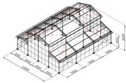
Atrium Tent Frame
